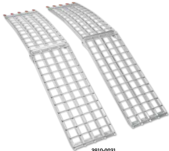
3910-0031 18" W X 95" L each; 2,500 lb. capacity
